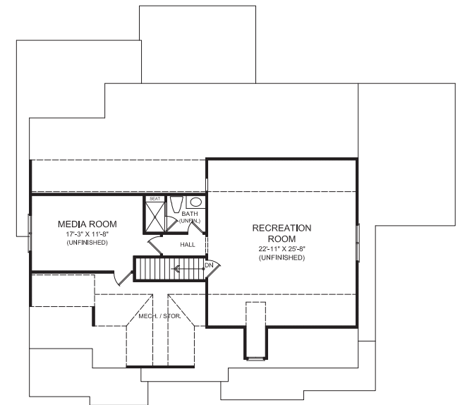
THIRD FLOOR
